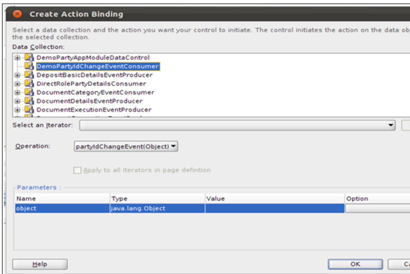
Figure 5–78 Create Action Binding
