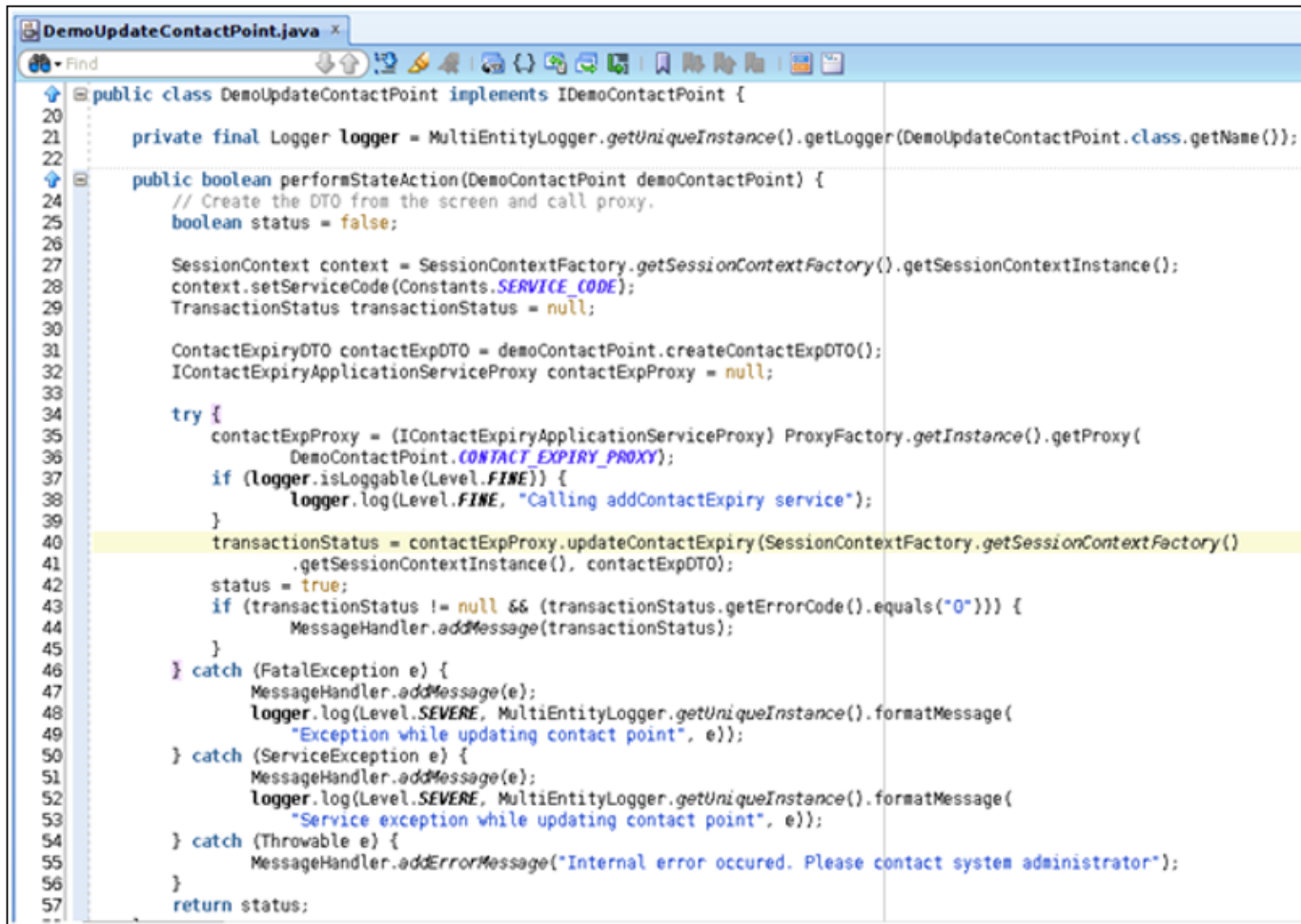
Figure 5–64 Create Update State Action Class
