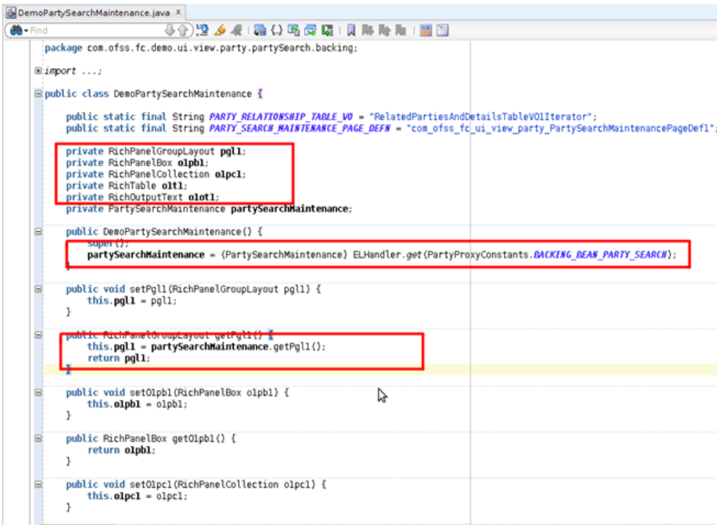
Figure 5–14 Creating Binding Bean Class
